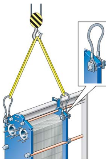
Lifting device for TK20-BW, T20-BW and T20-MW.
