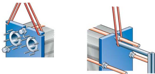
Lifting device for M6-MW and M10-BW.
