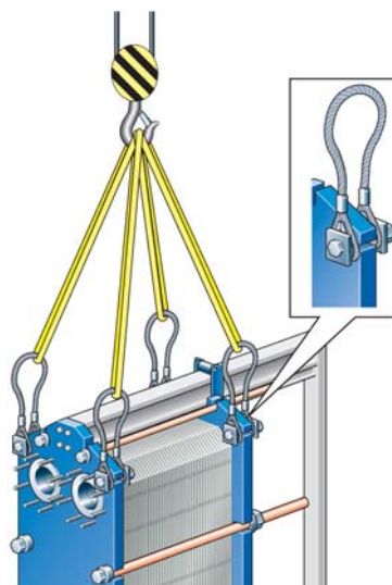
Lifting device for MA30-W.
